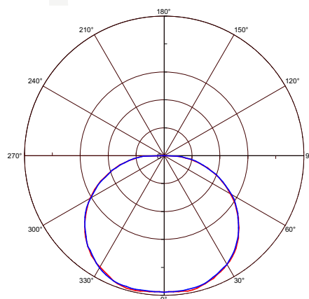
Planar Intensity Distribution Curve
