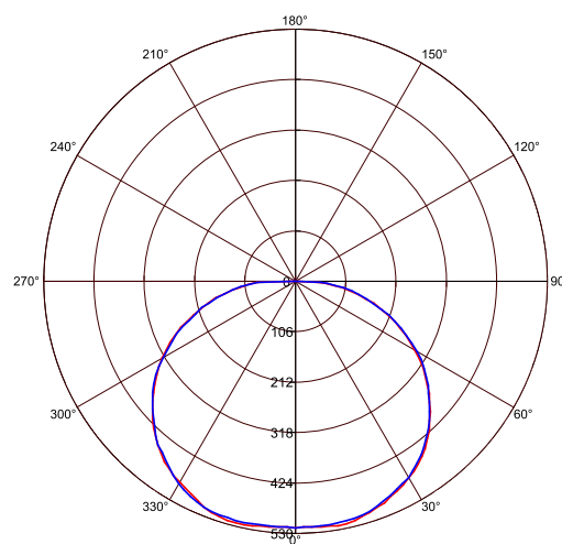
Planar Intensity Distribution Curve
